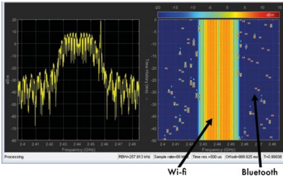
Spectral view of Bluetooth and WLAN coexistence (Image source: The MathWorks)
