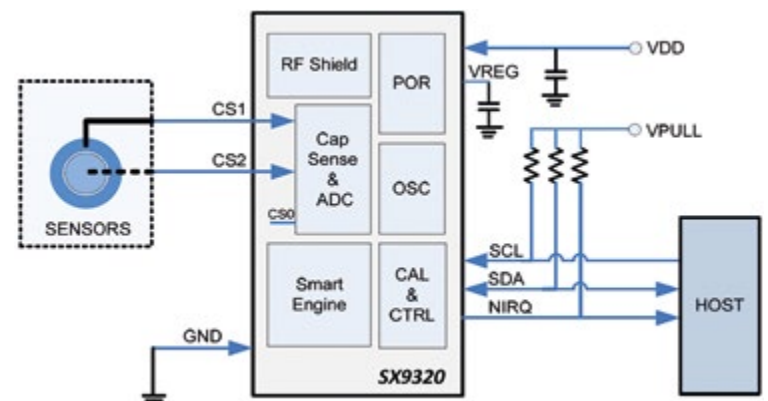
SAR Compliance for 5G Devices (Source: Semtech)
